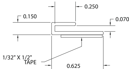
.045 WALL THICKNESS PROVISTA
