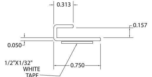
.050 WALL THICKNESS HIPS
