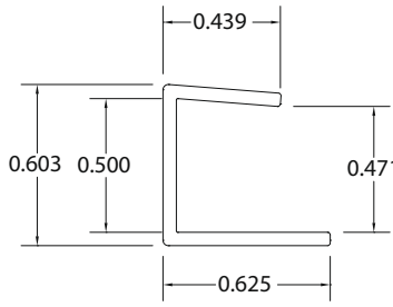
.050 WALL THICKNESS ABS
