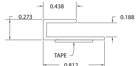
.045 WALL THICKNESS HIPS
