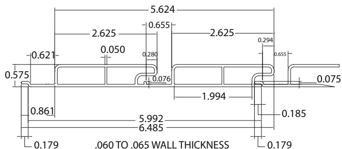
.060 TO .065 WALL THICKNESS
