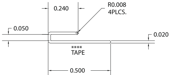
.020 WALL THICKNESS TRANSPARENT RPVC
