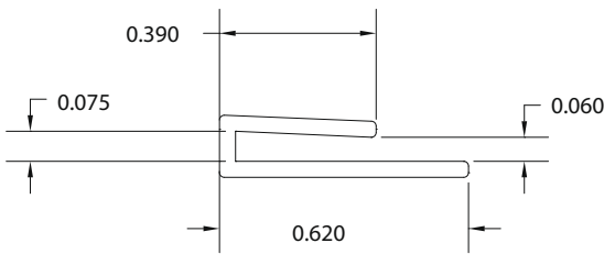
.040 WALL THICKNESS HIPS
