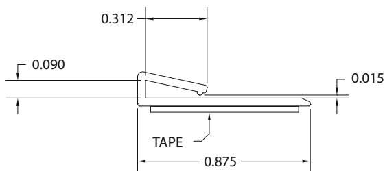
.050 WALL THICKNESS HIPS
